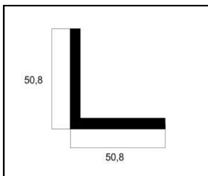
CT-033 CANTONEIRA 2 X 3/16 PESO: 1,392 Kg/m
